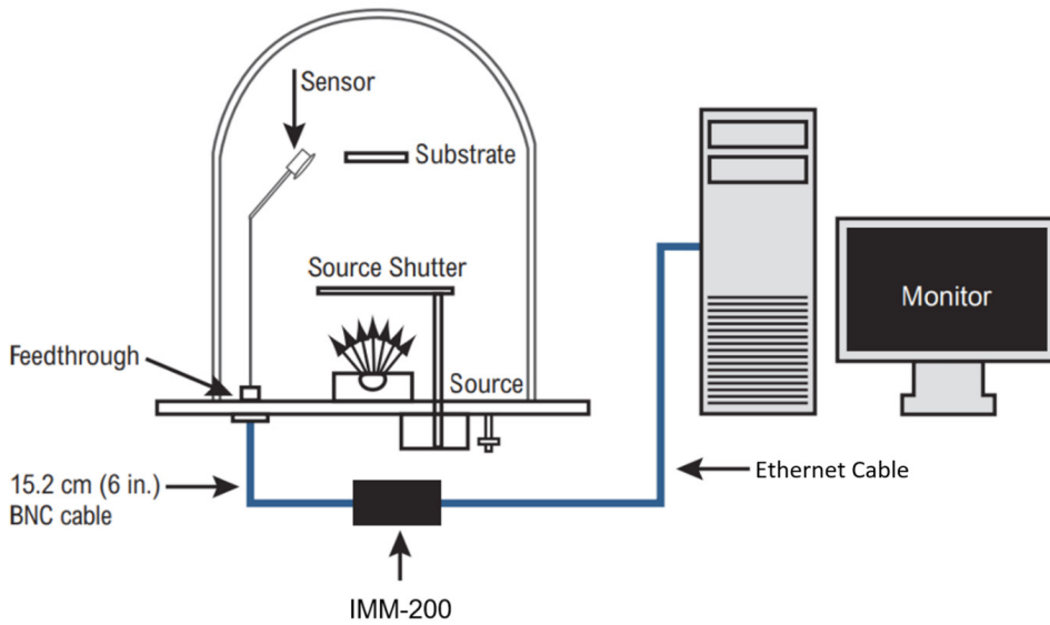
Typical IMM-200 installation
